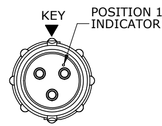
WIRE VIEW W8280-3PG-P-3XX SHOWN
