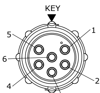
WIRE VIEW W8280-6PG-P-3XX
