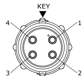
WIRE VIEW W8280-2PG-P-3XX
