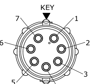
WIRE VIEW W8280-7PG-P-3XX
