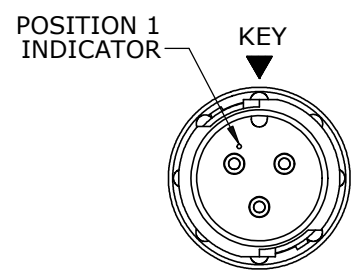
FACE VIEW W8280-3PG-P-3XX SHOWN
