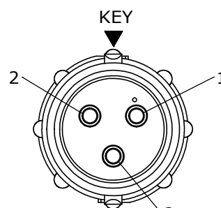
WIRE VIEW W8280-3PG-P-3XX
