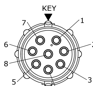
WIRE VIEW W8280-8PG-P-3XX
